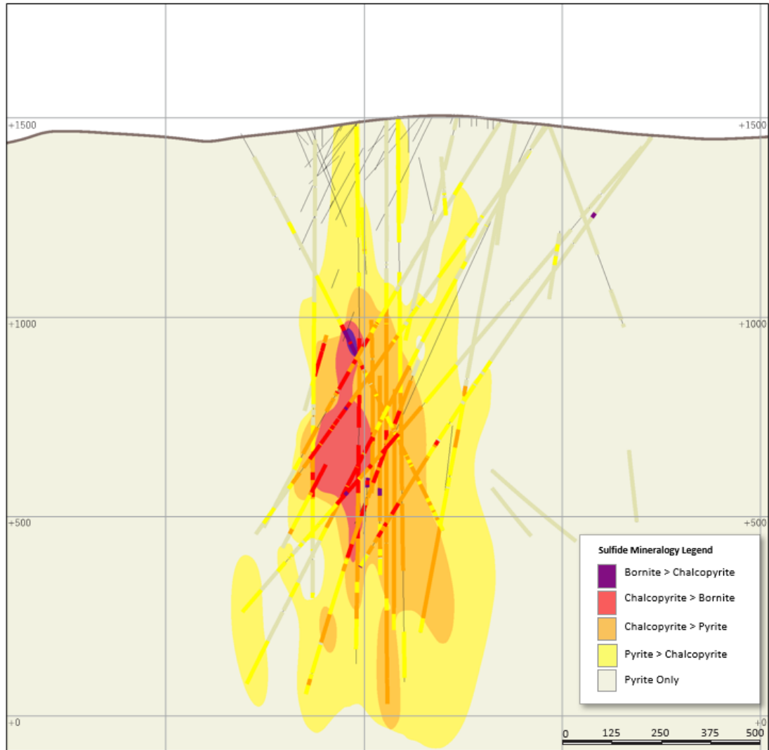
Figure 7-6: Red Chris Sulphide Speciation Model East Zone (Section 27N)
