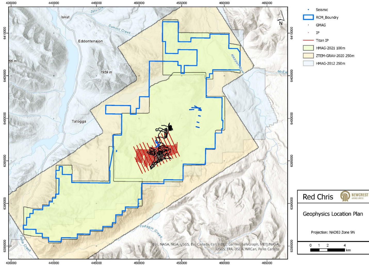
Figure 9-2: Geophysical Surveys
