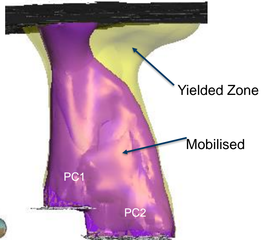
Cave shape as at January 2019
